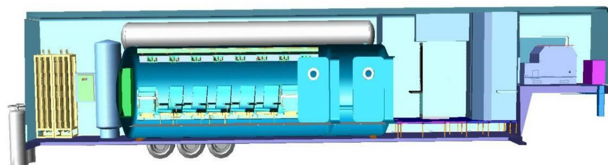
Dual Lock Chamber Layout - 12 place, 90" Diameter
