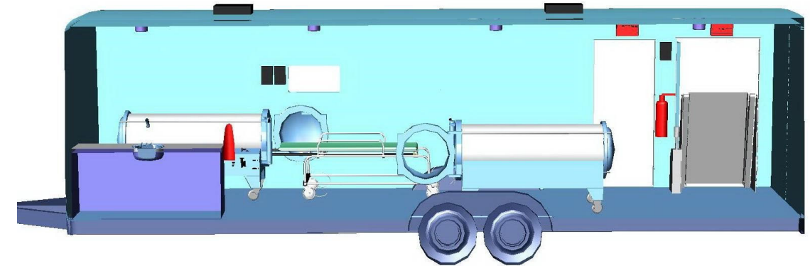
Views of two monoplace chambers placed in trailer
