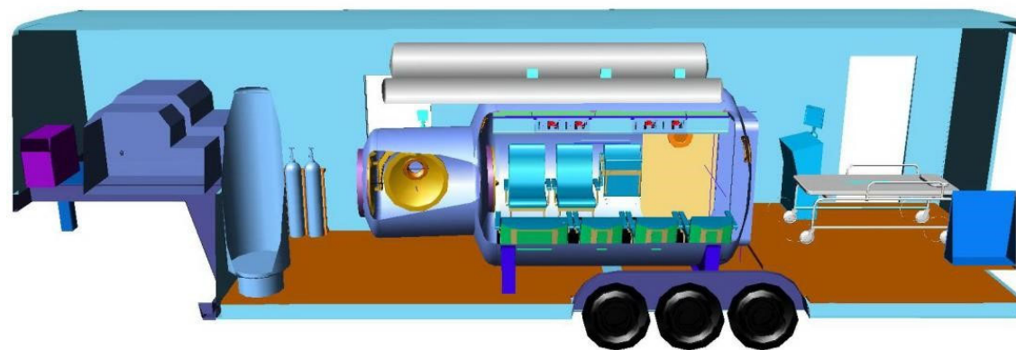
Dual Lock Chamber Layout - 6 place, 84" Diameter
